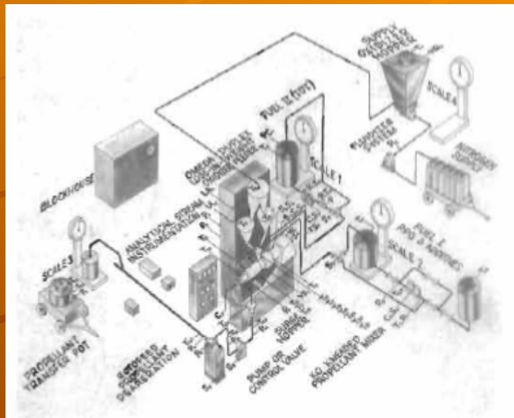
Figure 1-5B. Isometric pictorial flow diagram. By permission, J. W. Keating and R. D. Geckler, Aerojet General Corp.
