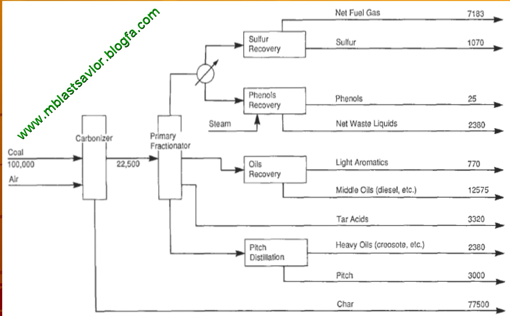
Coal carbonization block flowsheet. Quantities are in lb/hr
